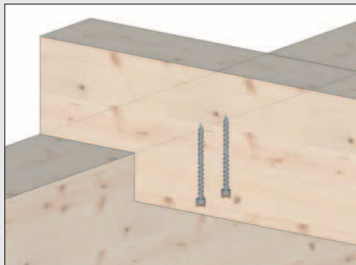
Common halving
