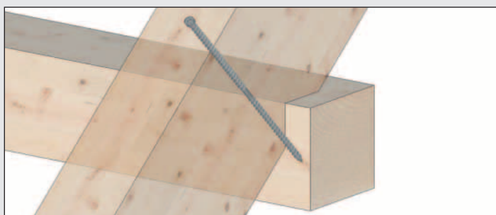
Rafter-purlin joints
